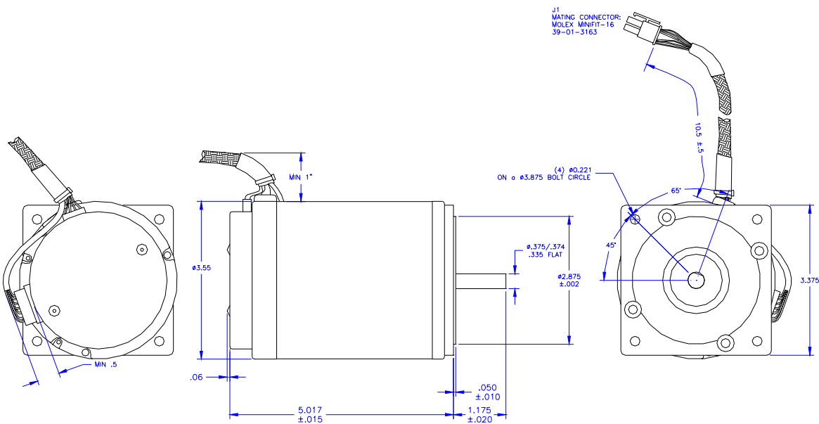
M-3450-FX motor with NEMA 34 flange
