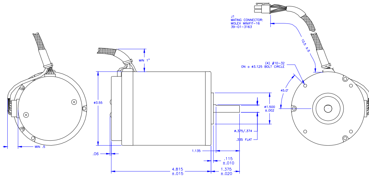
M-3450-XX motor without NEMA 34 flange
