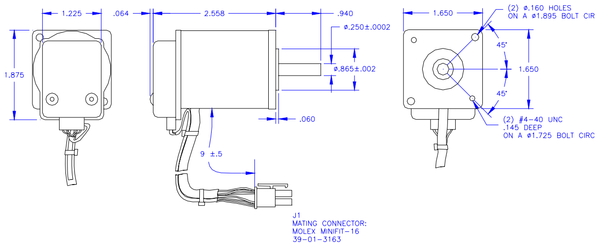
M-1726-FX: 4,000 counts/rev. with NEMA flange
