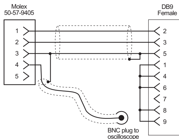
Typical Diagnostic/Configuration Cable (such as the Teknic SSt-DC)
