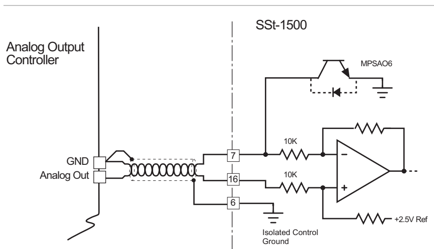
Analog Command Input Wiring
