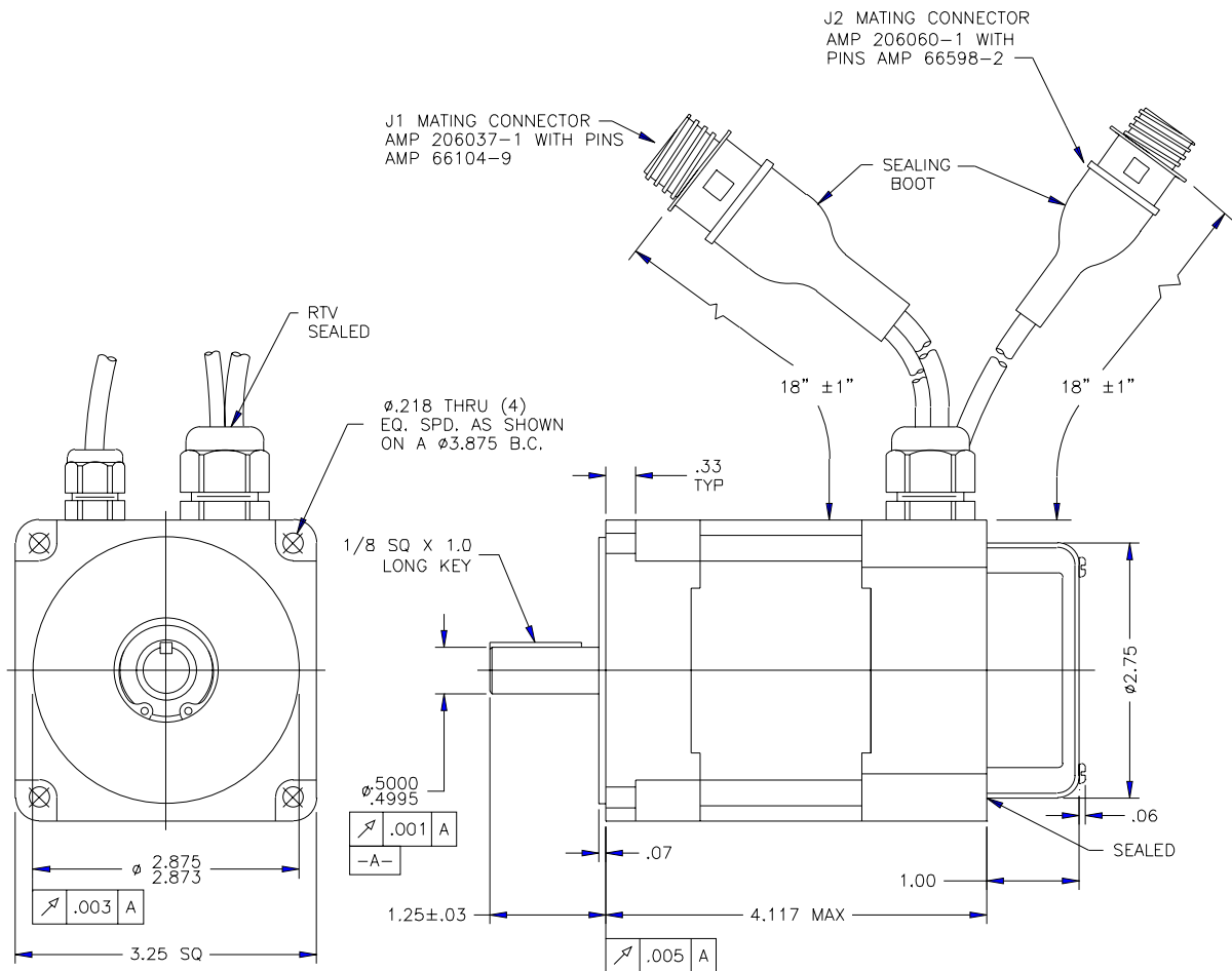
M-3462-FH sealed motor flange
