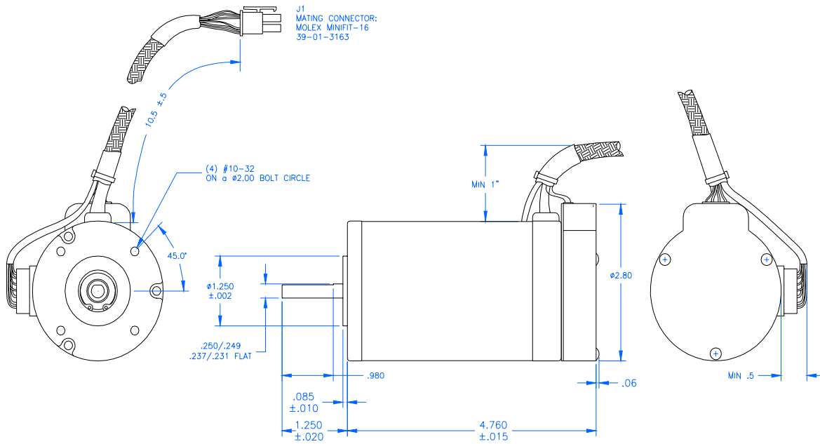
M-2348-XH: 8,000 counts/rev. without NEMA flange
